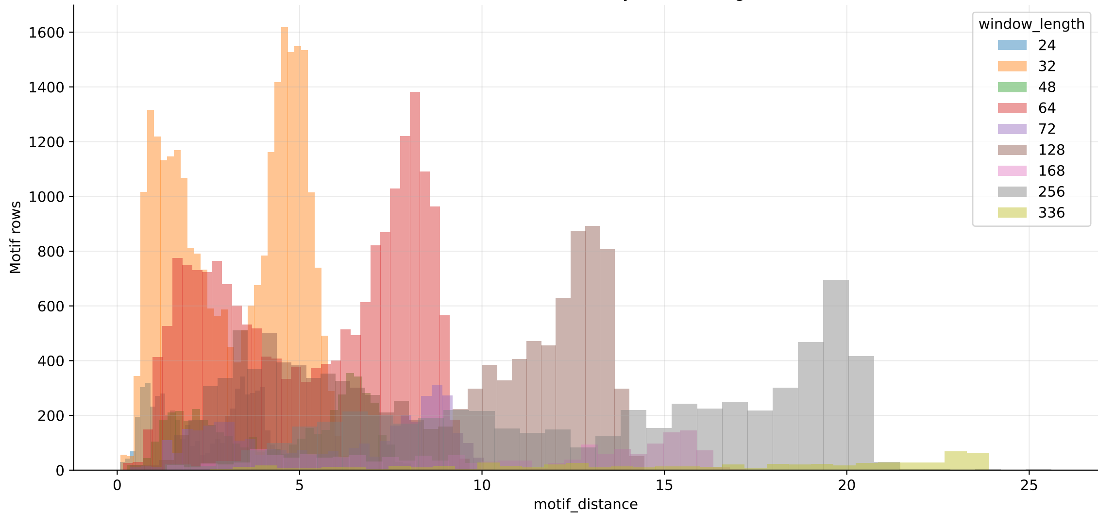
Matrix Profile distances by window length
